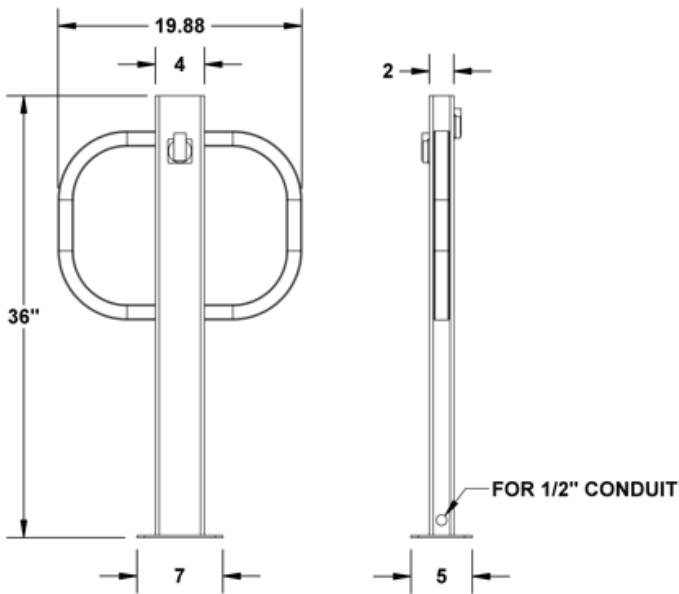
Locking Power Post
