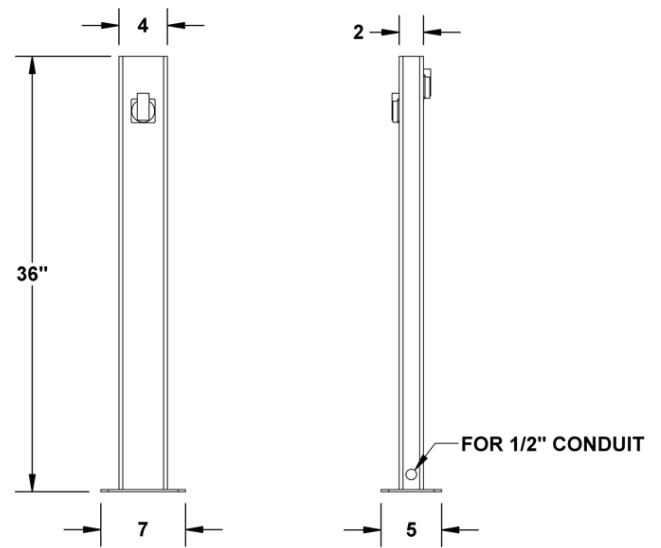
Non-locking Power Post
